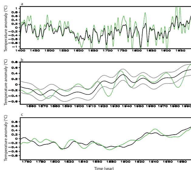
Fig. 1. Time series ( ^{\circ}\text{C} ) of the anomaly in annual mean surface temperature averaged over the 11 simulations using DA (black) for Scandinavia (defined here as the region 5^{\circ} – 35^{\circ} E, and 55 – 75^{\circ} N) and (a) the average of the 6 proxies used to constrain model results in this region (green), (b) the instrumental data compiled in the HadCRUT3 data set (green, Brohan et al., 2006), and (c) the average over Stockholm and Uppsala long instrumental time series, (Moberg et al., 2003). For (a), model results are averaged only over the points where proxy data are available. Reference period is 1850–1995. All the time series have been decadal smoothed. A 21-year running mean has been applied for panel (c).
