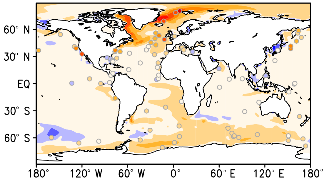
(a) SST change (Pliocene–pre-industrial)
