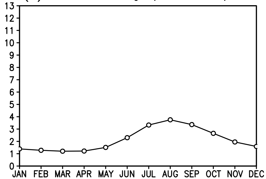
(c) Mean SST change (Arctic Ocean)
