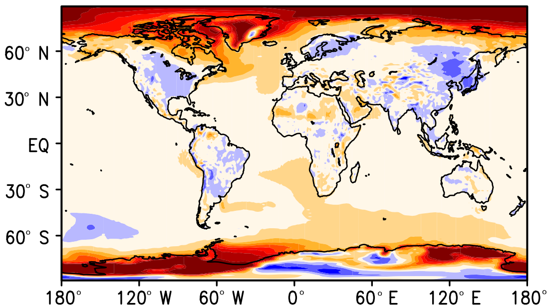
(b) SAT change (Pliocene–pre-industrial)
