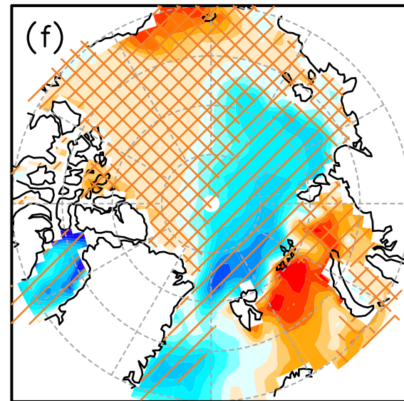
Net heat (Pliocene–pre-industrial)
