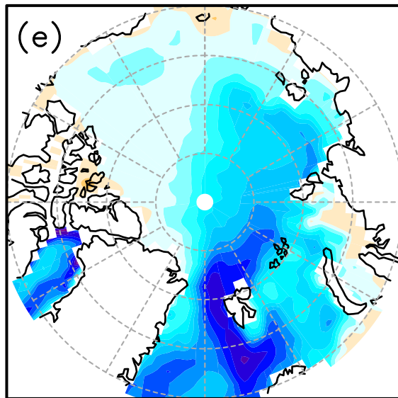
Net heat (Pliocene)
