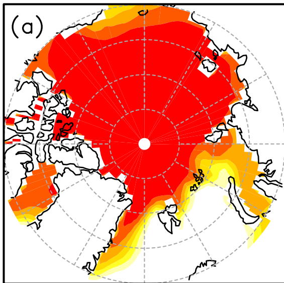
SIC (pre-industrial)
