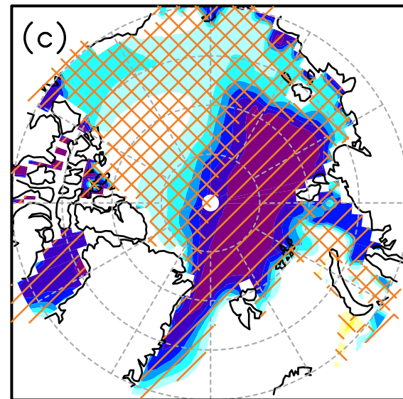
SIC (Pliocene–pre-industrial)
