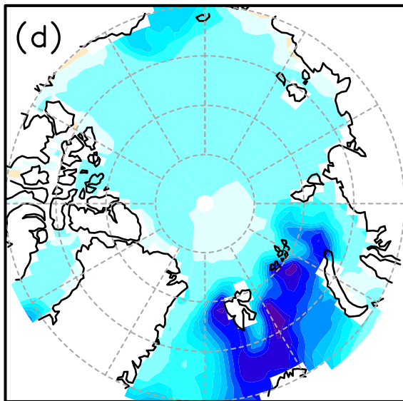
Net heat (pre-industrial)
