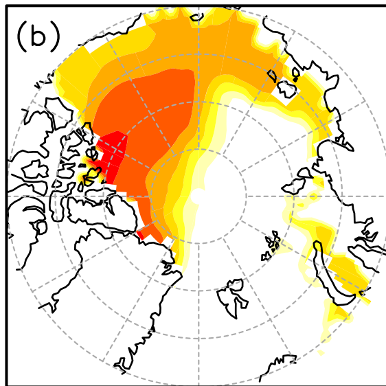
SIC (Pliocene)
