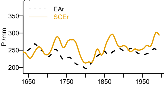
(c) Reconstructions
