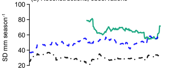
(a) Reconstructions, observations
