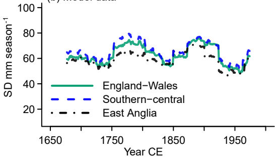
(b) Model data
